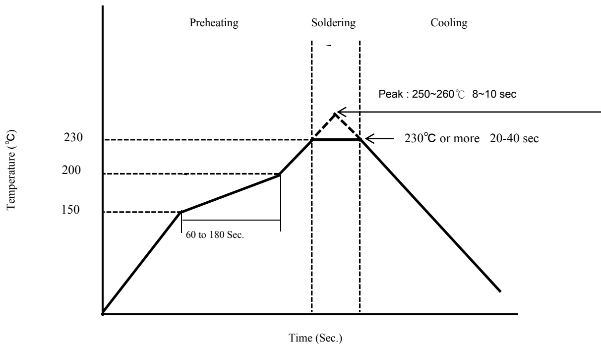
Figure 1. Re-flow Soldering
