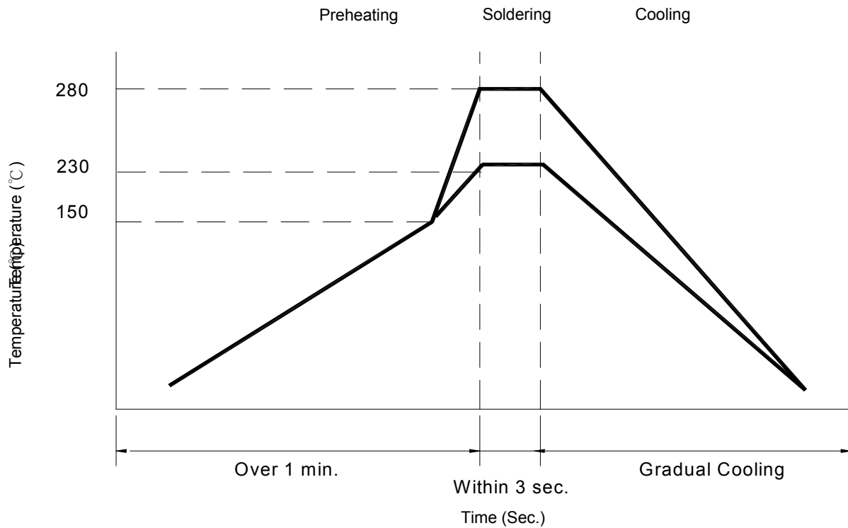
Figure 2. Hand Soldering
