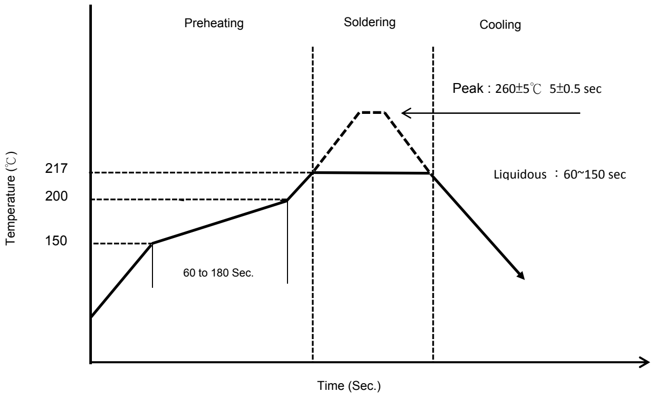
Figure 1. Re-flow Soldering
