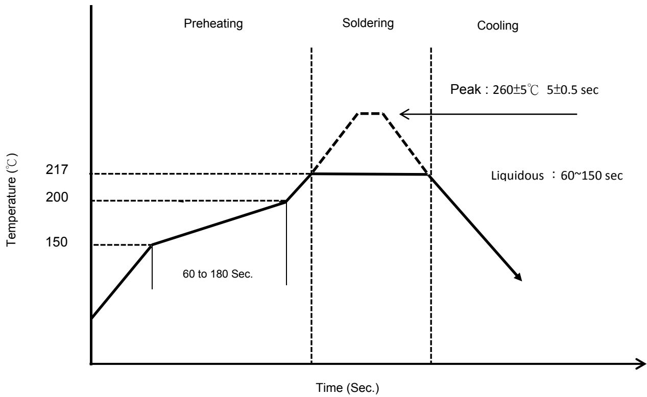
Figure 1. Re-flow Soldering
