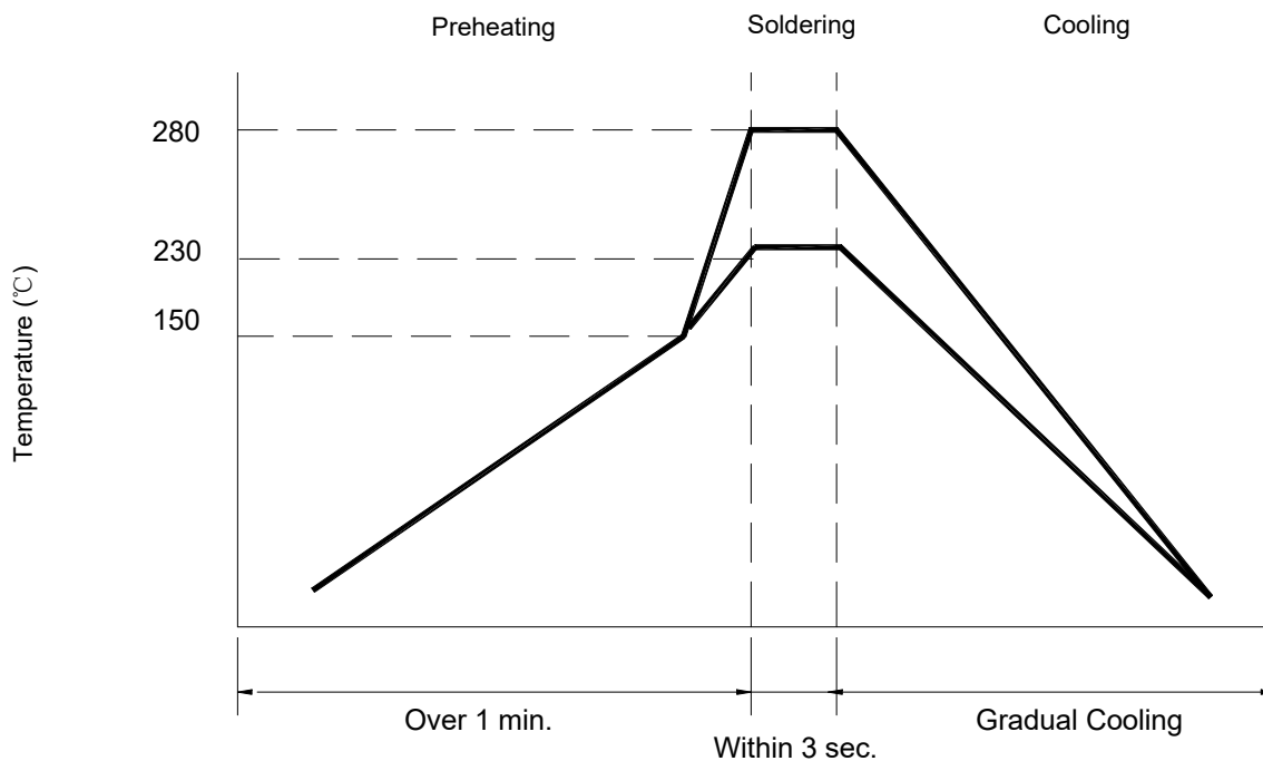
Figure 2. Hand Soldering
